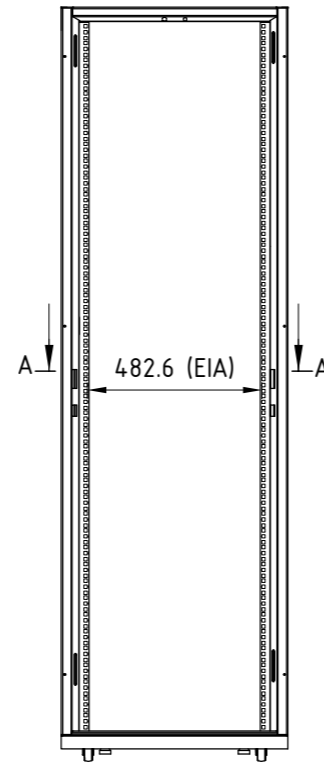
FRONT VIEW (REMOVE DOOR)
