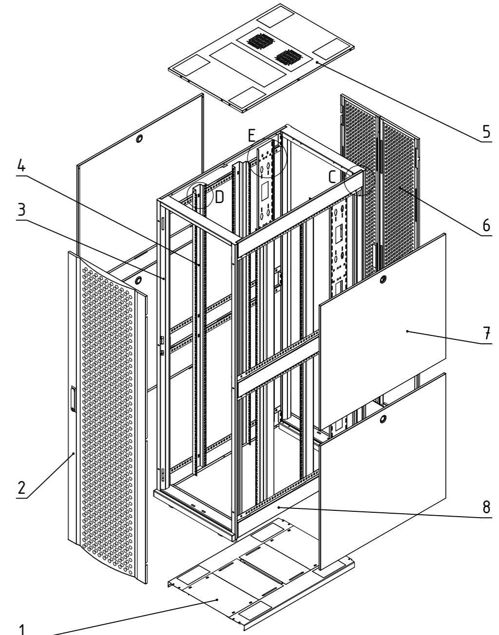
EXPLODED VIEW
