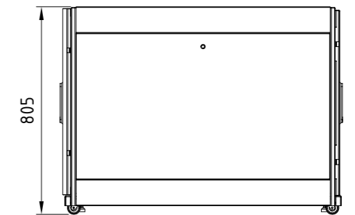
15U CABINET
