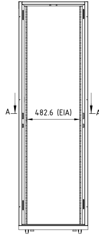
FRONT VIEW (REMOVE DOOR)
