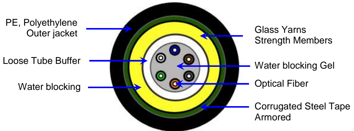
4-12 Fibers
